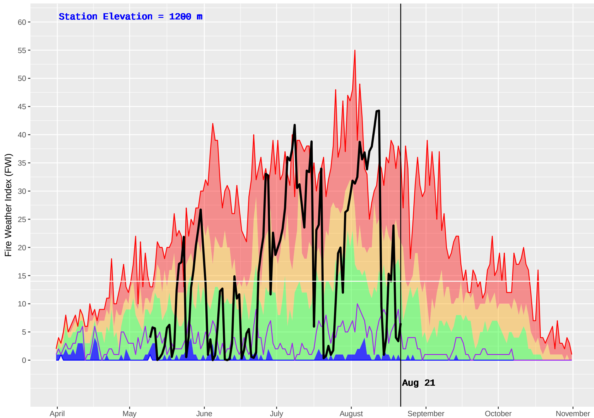
TSAR CREEK (361) : Historical (1986–2016) and Current (2017) Noon Fire Weather Index (FWI)
