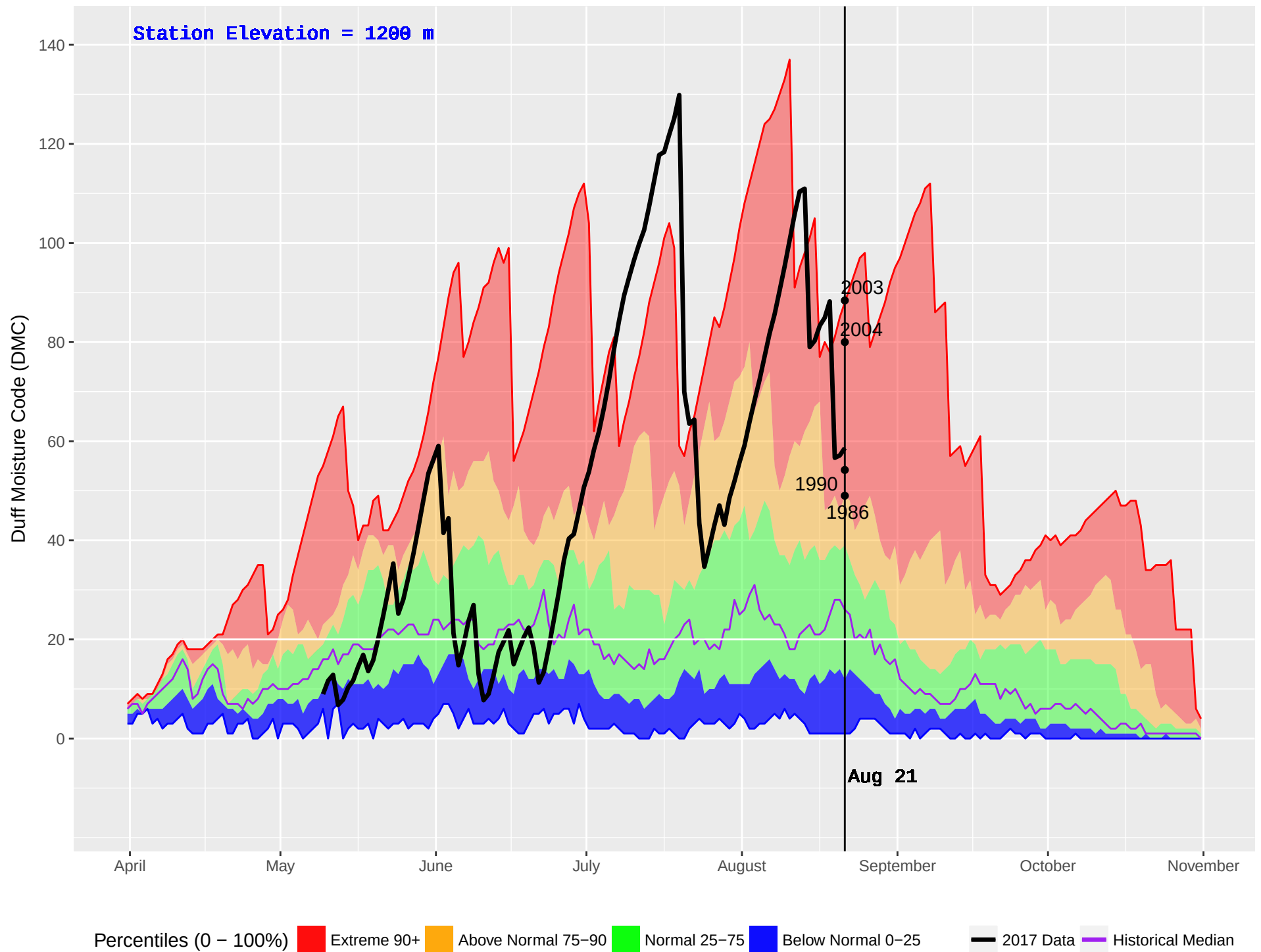
TSAR CREEK (361) : Historical (1986–2016) and Current (2017) Noon Duff Moisture Code (DMC)
